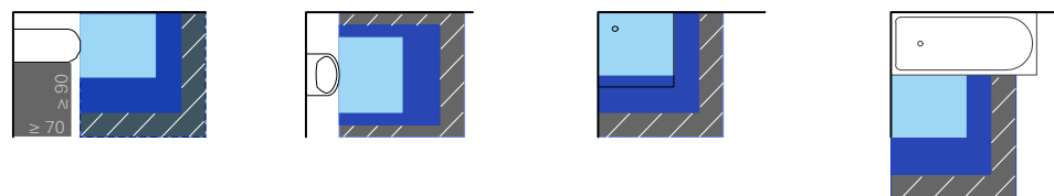
Abb. 15 Movement areas in front of sanitary fittings according to DIN 18022:1989-11, DIN 18025:1992-12 and DIN 18040:2011-09
