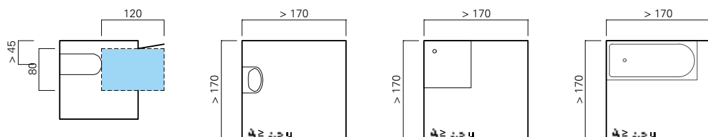
Abb. 16 Adaptable bathroom/shower according to SIA 500:2009, 10.2.1 Swiss requirements to be met by usable and movement areas for an obstacle-free WC or bathroom
