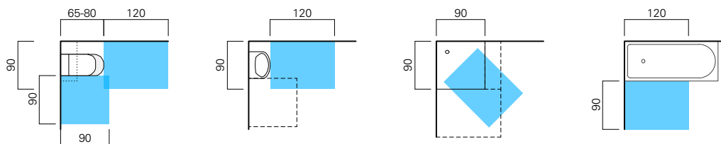
Abb. 17 Minimum size and requirements to be met by movement areas for a bathroom prepared so as to be accessible (ready)
