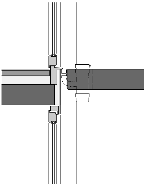
57 Detail Loggia M 1:20
