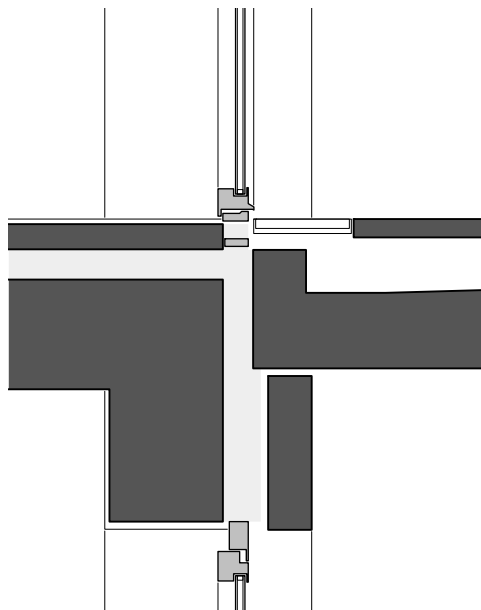
10 Detail Loggia M 1:20
