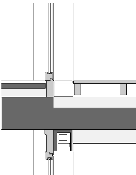
33 Detail Loggia M 1:20
